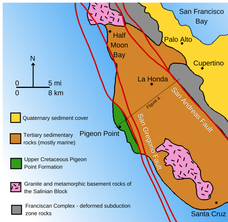
Figure 3. Geologic map of San Francisco Bay Area showing the Pigeon Point Formation and associated faults. Modified from Jaikla (2021).
